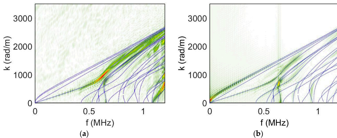
Figure 12. 2DFT (wavenumber k versus frequency f ) of simulated signals for the EPL3 specimen stimulated by sources D_1 ( M_x = 500 \text{ N}\cdot\mu\text{m}, 0 \text{ mm}, 0.1 \mu\text{s} ) (a), and D_2 ( M_x = 100 \text{ N}\cdot\mu\text{m}, 0.95 \text{ mm}, 1 \mu\text{s} ) (b).
