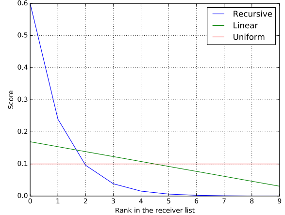
Fig. 6. Scores assigned by our 3 scoring functions f_U , f_L and f_R for a receiver list containing 10 users.
