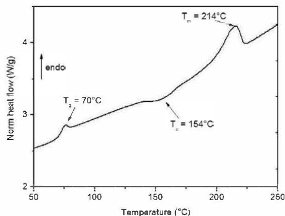
FIG. 3. PEKK oligomers DSC thermogram (heating rate 20°C min -1 ).
