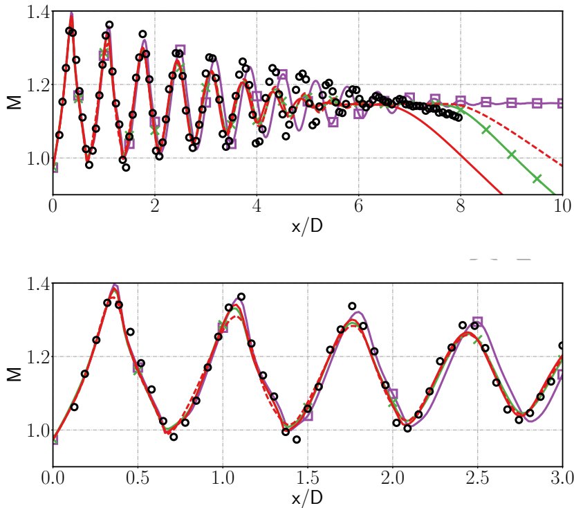
Figure 4 Mach number profile of the deterministic base case at the axis for different solvers and turbulence models. (a) full view, (b) detailed view. Red dashed line: 3D elsA, S-A. Red solid line: 2D-axi Fluent S-A. Green solid line: 2D-axi Fluent k - \varepsilon . Purple solid line: 2D-axi Fluent k - \omega . Symbols: Experimental data.
