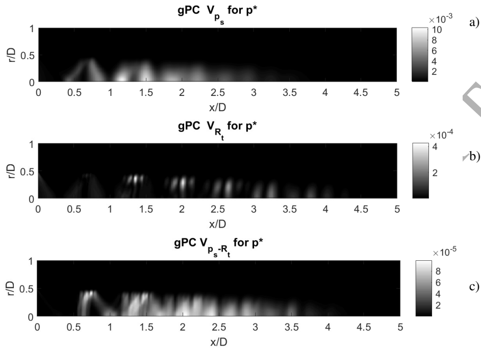
Figure 20 Contribution to the total variance of a) stagnation pressure, b) laminar to turbulent viscosity ratio and c) their interaction, for p^* .
