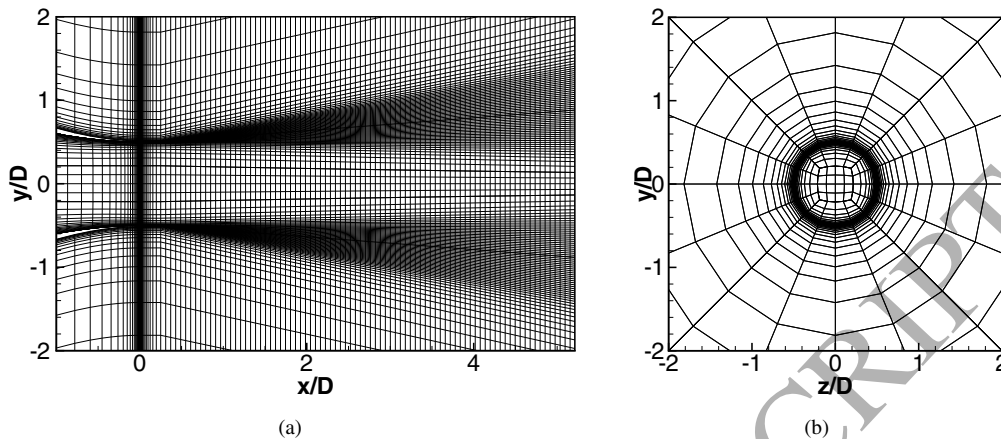
Figure 1 Mesh cuts representing every fourth cells in the plane (a) z/D = 0 and the plane (b) x/D = 0 .
