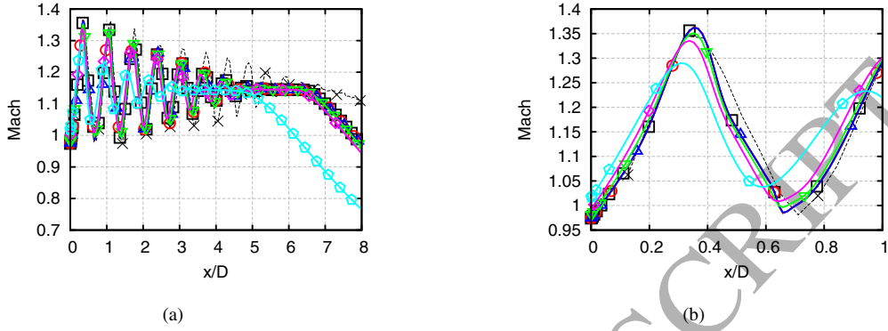
Figure 5 Mach number profile of the deterministic base case at the centreline for different R_t inlet values in a (a) general and a (b) detailed view. Experimental ×, R_t = 0.022 □, R_t = 0.22 ○, R_t = 2.2 △, R_t = 22 ▽, R_t = 220 ◇, R_t = 2200 ◇.
