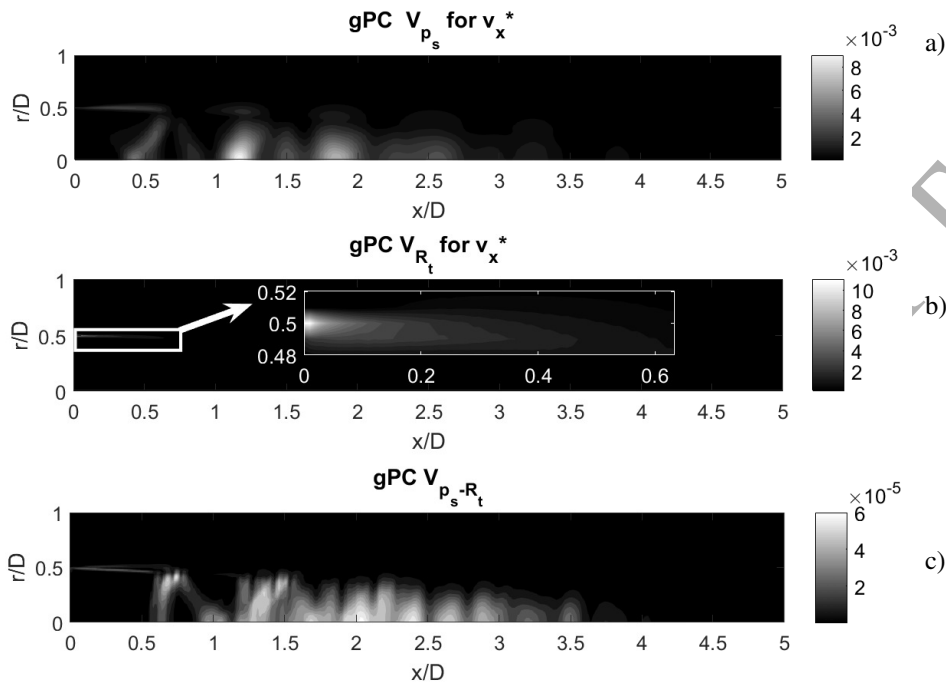
Figure 18 Contribution to the total variance of a) stagnation pressure, b) laminar to turbulent viscosity ratio and c) their interaction, for v_x^* .
