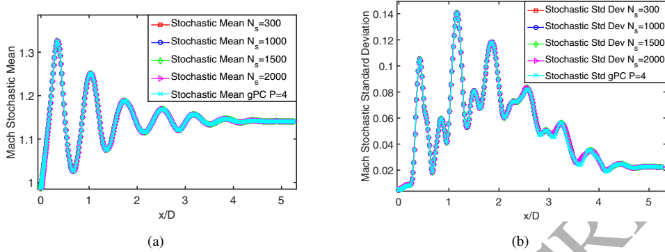
Figure 10 Evolution of the Mach stochastic means (a) and standard deviations (b) along the centerline for LHS on Kriging surrogates for different number of samples and its comparison with gPC results. Even for a small number of samples, LHS is undergoing very good convergence.
