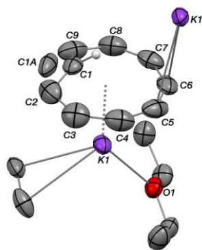
Figure 1. Molecular structure of KL 1 •OEt 2 recorded at 150 K; thermal ellipsoids are shown at 50% probability. C1 and C1A show the positional disorder. Hydrogen atoms have been removed for clarity except that of C1 in order to show its orientation.
