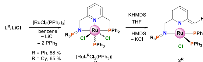
Scheme 2: Coordination of \text{L}^{\text{Ph}} and \text{L}^{\text{Cy}} to [\text{RuCl}_2(\text{PPh}_3)_3] and benzylic deprotonation
