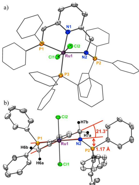
Figure 2: Thermal ellipsoid plots of [\text{Ru}^{\text{L}^{\text{Ph}}}\text{Cl}_2(\text{PPh}_3)] ( \mathbf{1}^{\text{Ph}} ): (a) perspective; (b) In the \text{P3N1} direction (with \text{PPh}_3 ligand omitted). Unless depicted, hydrogen atoms were omitted; some phenyl groups were depicted in a wire-frame model for clarity. Selected bond lengths (Å) and angles ( ^\circ ): \text{N2}-\text{P2} 1.600(2), \text{N2}-\text{Ru1} 2.249(2), \text{P1}-\text{Ru1} 2.2537(7), \text{N1}-\text{Ru1} 2.103(2), \text{P3}-\text{Ru1} 2.3545(7), \text{Cl1}-\text{Ru1} 2.4168(7), \text{Cl2}-\text{Ru1} 2.4169(7), \text{N2}-\text{Ru1}-\text{P1} 156.42(6), \text{N1}-\text{Ru1}-\text{P3} 171.64(7), \text{Cl1}-\text{Ru1}-\text{Cl2} 175.74(3), \text{N2}-\text{Ru1}-\text{N1} 75.6(1), \text{P1}-\text{Ru1}-\text{N1} 80.98(7), \text{P3}-\text{Ru1}-\text{N2} 100.78(6), \text{P3}-\text{Ru1}-\text{P1} 102.80(3), \text{N1}-\text{Ru1}-\text{Cl1} 88.47(7), \text{N2}-\text{Ru1}-\text{Cl1} 91.10(6), \text{P1}-\text{Ru1}-\text{Cl1} 85.20(3), \text{P3}-\text{Ru1}-\text{Cl1} 99.22(3), \text{N1}-\text{Ru1}-\text{Cl2} 87.29(7), \text{N2}-\text{Ru1}-\text{Cl2} 88.19(6), \text{P1}-\text{Ru1}-\text{Cl2} 93.78(3), \text{P3}-\text{Ru1}-\text{Cl2} 85.03(3).
