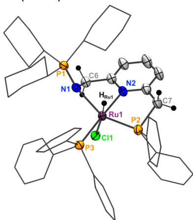
Figure 6. Thermal ellipsoids plot of [\text{RuL}^{\text{Cy}}\text{HCl}(\text{PPh}_3)] ( 3^{\text{Cy}} ); \text{H}_{\text{Ru1}} was located on the density map and refined isotropically. Hydrogen atoms, unless depicted were omitted, cyclohexyl and phenyl groups are depicted in a wire-frame model for clarity. Only one of the two independent molecules 3^{\text{Cy}} occurring in the asymmetric unit is presented. Selected bond lengths (Å) and angles (°): N1-P1 1.612(3), \text{H}_{\text{Ru1}}-\text{Ru1} 1.57(5), N1-Ru1 2.269(3), P2-Ru1 2.217(1), N2-Ru1 2.107(4), P3-Ru1 2.276(1), Cl1-Ru1 2.603(1); N1-Ru1-P2 154.61(9), \text{H}_{\text{Ru1}}-\text{Ru1}-\text{Cl1} 175(2), P3-Ru1-N2 176.3(1), N1-Ru1-N2 75.3(1), P2-Ru1-N2 82.0(1), Cl1-Ru1-N1 87.32(9), Cl1-Ru1-P2 102.51(4), N2-Ru1-Cl1 86.3(1), N1-Ru1-P3 105.70(9), P2-Ru1-P3 97.70(4), Cl1-Ru1-P3 90.18(4), N1-Ru1- \text{H}_{\text{Ru1}} 89(2), N2-Ru1- \text{H}_{\text{Ru1}} 96(2), P2-Ru1- \text{H}_{\text{Ru1}} 82(2), P3-Ru1- \text{H}_{\text{Ru1}} 87(2).
