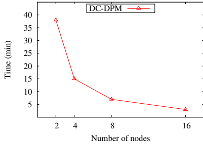
Figure 6: Clustering time as a function of the number of computing nodes on the image of our use-case.
