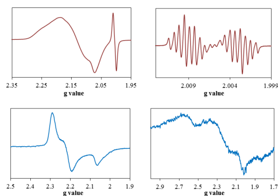
Figure 7. EPR spectra of [Ni(Psalen OMe )](SbF 6 ) (top: left at 10K, right at 290 K) and [Ni(Psalen fbu )](SbF 6 ) (bottom: left at 5 K, right at 252 K) in CH 2 Cl 2 solution.
