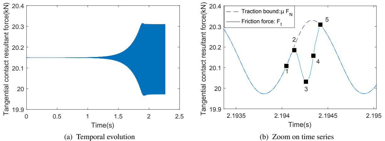
Figure 13: Tangential contact resultant force. The status of the contact points at the time steps marked with Arabic numerals is represented Fig. 14
