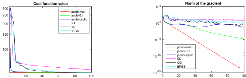
FIG. 1. Cost function and norm of the gradient, Example 1
