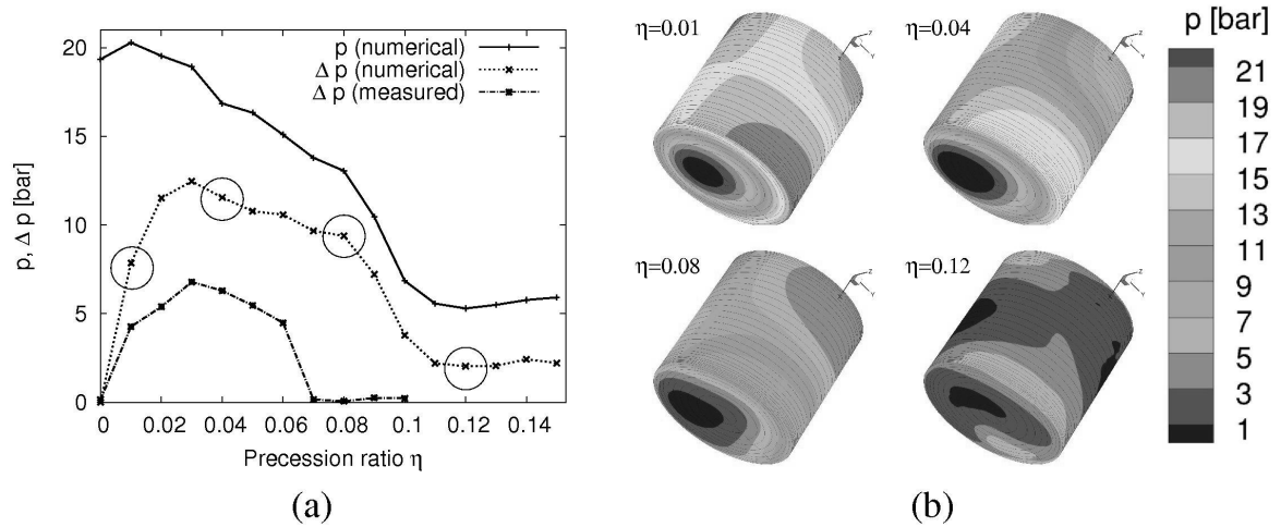
Figure 1: Pressure values for a precessing cylinder with 90^\circ angle between rotation and precession axes. (a) Maximum pressure p (numerically determined at Re=6680 ) and pressure pulsation amplitude \Delta p (numerical and experimental) when scaled to the large device. (b) Pressure distribution (numerical) for 4 specific precession ratios.
