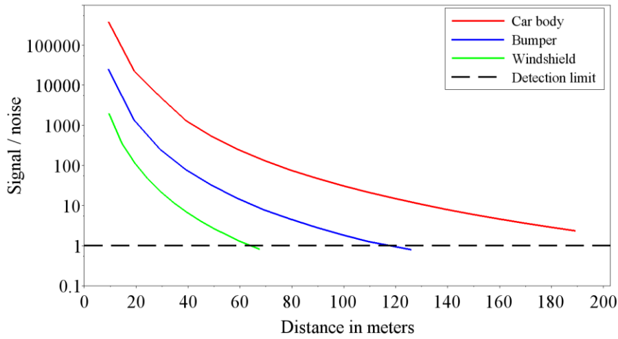
Figure 3: Variation of the signal/noise as a function of the distance between LIDAR and car target. Red curve: body car; Blue curve: bumper; Green curve: windshield; Black dashed line: detection limit
