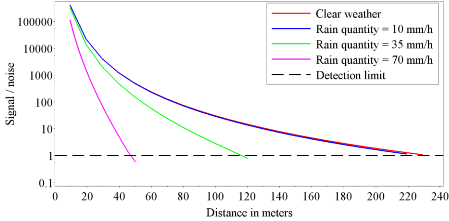
Figure 5: Variation of the signal/noise of the central LASER beam as a function of the rain quantity and distance between LIDAR and car target. The laser beam is focalized on the metal body car and the raindrop radius is equal to 3 mm.
