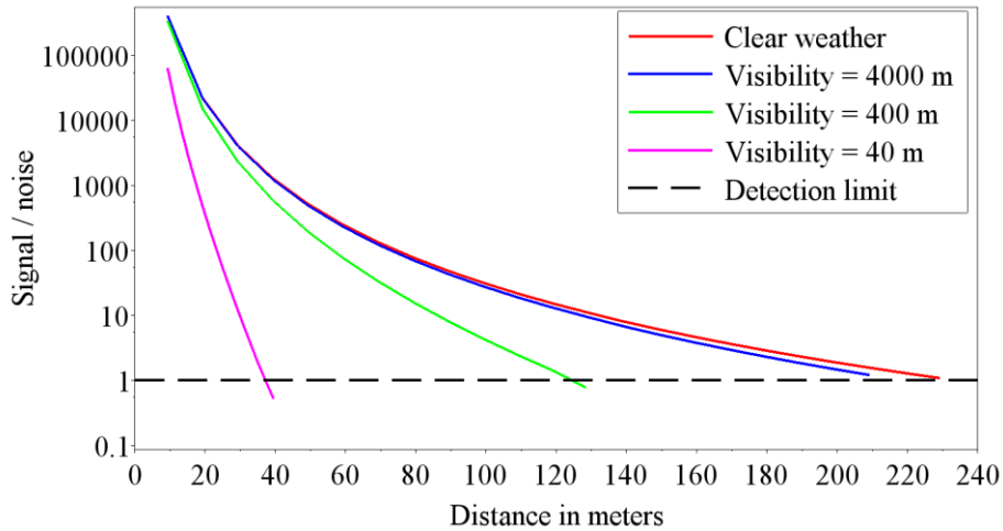
Figure 4: Variation of the signal/noise of the central LASER beam as a function of the fog visibility and distance between LIDAR and car target. The laser beam is focalize on the metal body car.
