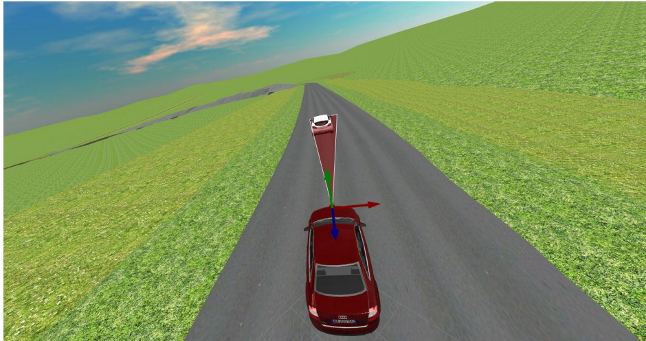
Figure 2: Reflectivity calculation example: The white car is stationary while the red car is in approaching, the LIDAR is placed in the front bumper and is focalized on the car body.
