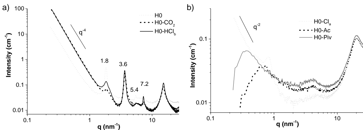
Figure 1. SAXS profiles of the a) H0, H0-Cl b and H0-CO 2 materials; b) H0-Cl a , H0-Ac and H0-Piv solutions.
