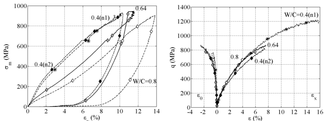
Fig. 14. Triaxial tests at 650 MPa confinement for concretes EC06 (full line with grey symbols), EC08 (dash-dot line with white symbols) and EC04 (n2: dash line with black symbols; n1: dash-dot line with asterisk symbols *); (a) Mean stress \sigma_m vs. volumetric strain \epsilon_v ; (b) Stress deviator q vs. strain components \epsilon_x and \epsilon_\theta
