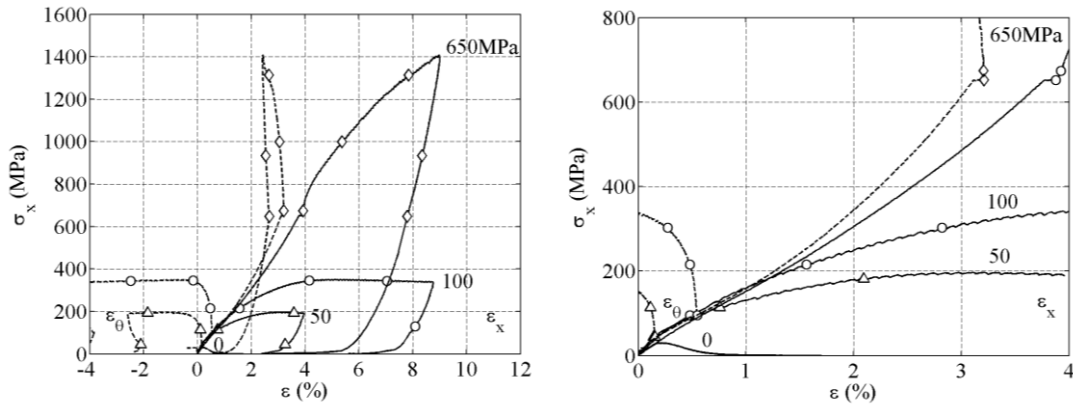
Fig. 8. Triaxial tests conducted at different confining pressures p on concrete EC08 (W/C=0.80): Axial stress \sigma_x vs. strain components \epsilon_x and \epsilon_\theta ; p = 0 MPa (no marker); 50 MPa (triangle); 100 MPa (circle); 650MPa (diamond); axial strain \epsilon_x (full line); circumferential strain \epsilon_\theta (dash line). Zoom on the hydrostatic phases of the loading (figure on the right).
