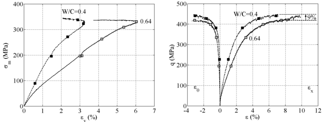
Fig. 13. Triaxial tests at 200 MPa confinement for concretes EC04 (dash line with black symbols) and EC06 (full line with grey symbols); (a) Mean stress \sigma_m vs. volumetric strain \epsilon_v ; (b) Stress deviator q vs. strain components \epsilon_x and \epsilon_\theta
