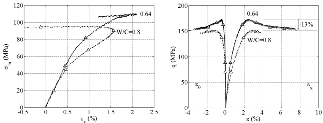
Fig. 11. Triaxial tests run at 50 MPa confinement for concretes EC06 (full line with grey symbols) and EC08 (dash-dot line with white symbols); (a) Mean stress \sigma_m vs. volumetric strain \epsilon_v (b) Stress deviator q vs. strain components \epsilon_x and \epsilon_\theta
