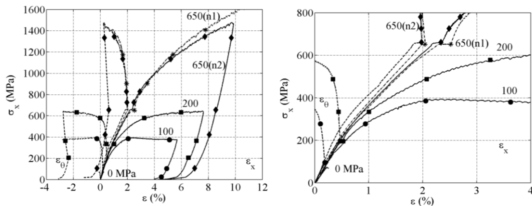
Fig. 10. Triaxial tests conducted at different confining pressures p on concrete EC04 (W/C = 0.4): Axial stress \sigma_x vs. strain components \epsilon_x and \epsilon_\theta ; p = 0 MPa (no marker); 100 MPa (circle); 200 MPa (square); 650 MPa (n2) (diamond); 650 MPa (n1) (*, dash-dot line). Zoom on the hydrostatic phases of the loading (figure on the right).
