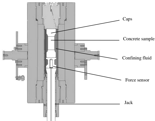
Figure 2: Cross-section view of the confining cell
