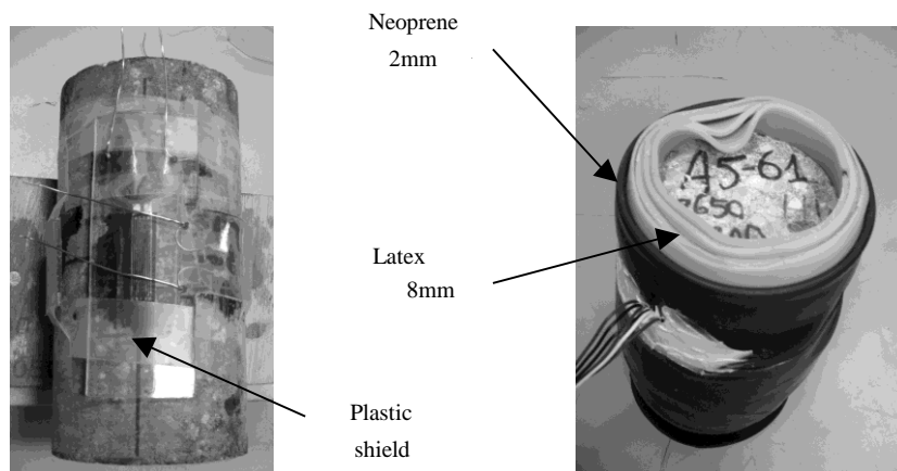
Figure 5: Protective device placed around the sample: Plastic shield (left photograph) and multilayer membrane (right)
