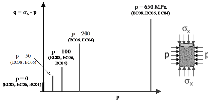
Fig. 6. Loading path of the completed tests: deviatoric stress q vs. confining pressure p ; \sigma_x : axial stress; EC08: W/C=0.8; EC06: W/C=0.64; EC04: W/C=0.4
