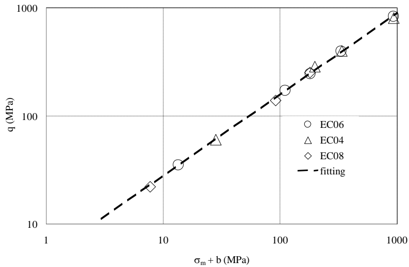
Figure 17: Limit states of concretes EC04, EC06 and EC08: \log(q) vs. \log(\sigma_m+b) ; EC06 b=1.82 MPa (o); EC04 b=8 MPa( \Delta ); EC08 b=0.4 MPa ( \diamond ); power law fitting q= a(b+\sigma_m)^c where a= 4.81 MPa ^{1-c} and c=0.758 (dash line)
