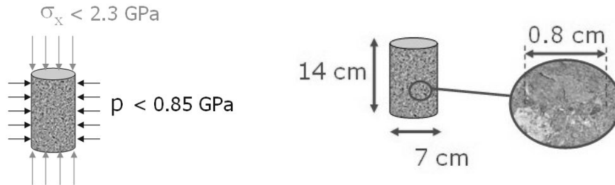
Figure 3: Maximum press capacity and associated sample sizes of the triaxial cell
