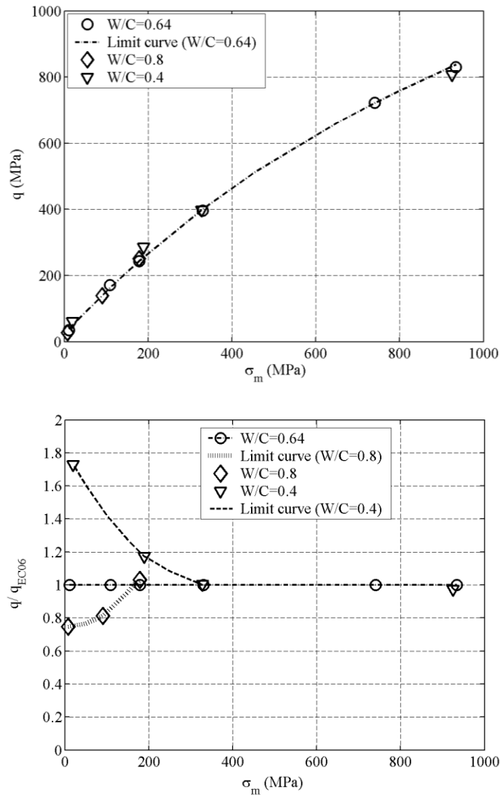
Fig. 15. Limit states of concretes EC04, EC06 and EC08: (a) Deviatoric stress q vs. mean stress \sigma_m (b) Relative deviator q/q_{EC06} vs. mean stress \sigma_m , where q_{EC06} is the deviatoric stress associated with the limit state of reference concrete EC06
