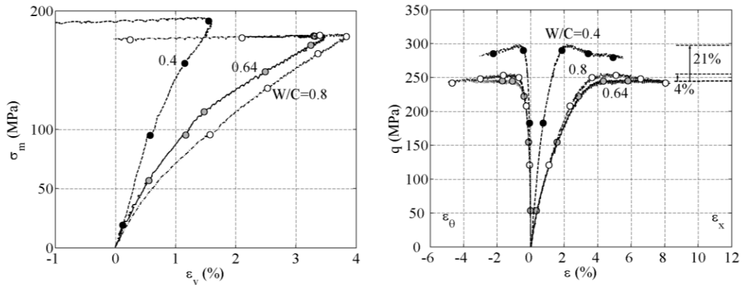
Fig. 12. Triaxial tests at 100 MPa confinement for concretes EC04 (dash line with black symbols), EC06 (full line with grey symbols), EC08 (dash-dot line with white symbols); (a) Mean stress \sigma_m vs. volumetric strain \epsilon_v ; (b) Stress deviator q vs. strain components \epsilon_x and \epsilon_\theta
