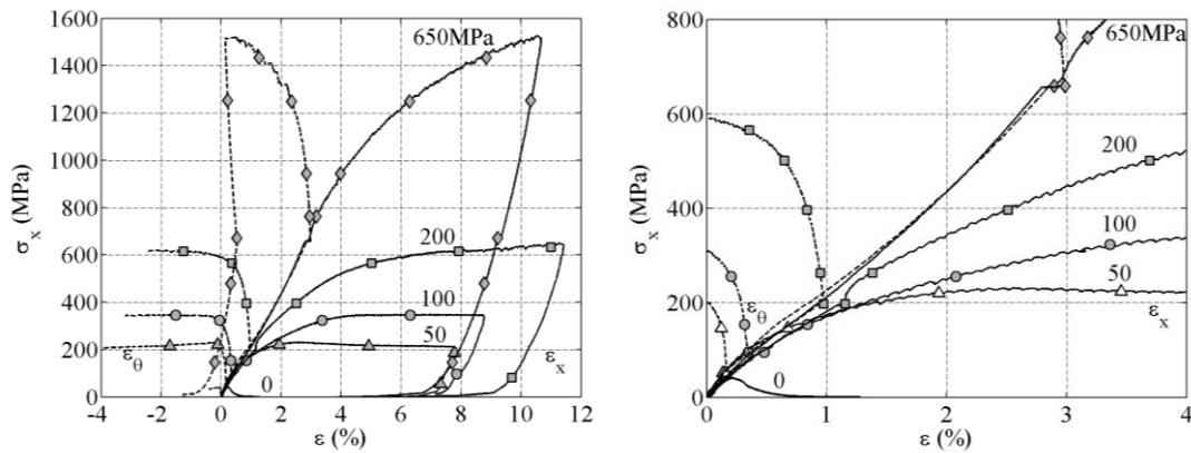
Fig. 8. Triaxial tests conducted at different confining pressures p on concrete EC06 (W/C=0.64): Axial stress \sigma_x vs. strain components \epsilon_x and \epsilon_\theta ; p = 0 MPa (no marker); 50 MPa (triangle); 100 MPa (circle); 200 MPa (square); 650MPa (diamond); axial strain \epsilon_x (full line); circumferential strain \epsilon_\theta (dash line). Zoom on the hydrostatic phases of the loading (figure on the right).
