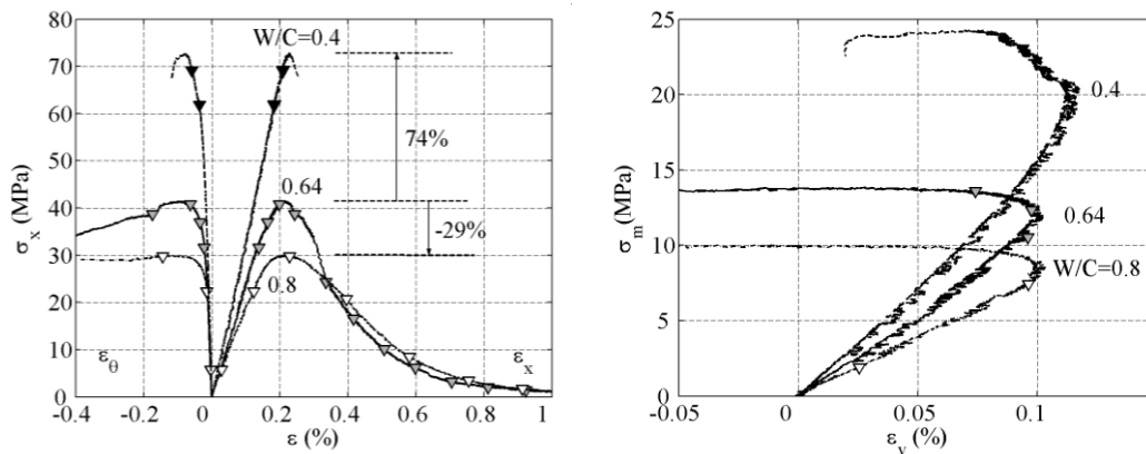
Fig. 7. Unconfined compression tests: EC08 (white symbols), EC06(grey symbols) and EC04 (black symbols); (a) Axial stress \sigma_x vs. strain components \epsilon_x and \epsilon_\theta (b) Mean stress \sigma_m vs. vol. strain \epsilon_v
