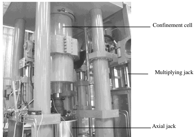
Figure 1: General view of the GIGA press
