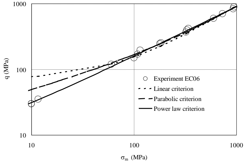
Figure 16: Comparison between the limit states of the EC06 concrete and the most common concrete criteria; experiment EC06 (o); linear criterion q=b+c\sigma_m (dot line); parabolic criterion q=(a+b\sigma_m+c\sigma_m^2)^{1/2} (dash line); power law criterion q= a(b+\sigma_m)^c (full line)
