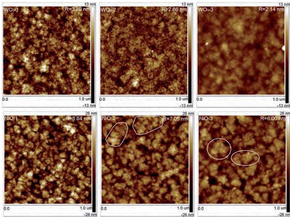
Fig. 6 AFM images of disassembled non-cycled and cycled cathodic ( \text{WO}_3 -1 and \text{WO}_3 -2, \text{WO}_3 -3 respectively) and anodic EC (NiO-1 and NiO-2, NiO-3 respectively) films (roughness values are shown; agglomeration evolution in degraded films is marked with white circles).
