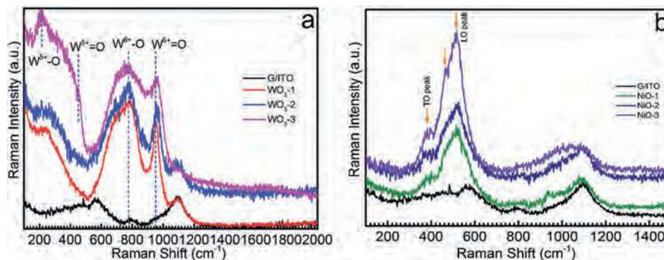
Fig. 5 Raman spectra of disassembled non-cycled and cycled (a) cathodic ( \text{WO}_3 -1 and \text{WO}_3 -2, \text{WO}_3 -3 respectively) and (b) anodic EC (NiO-1 and NiO-2, NiO-3, respectively) films.
