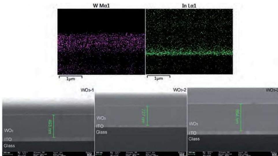
Fig. 7 Typical cross-view EDS-elemental mapping and SEM image of the FIB-cut sample for disassembled cathodic \text{WO}_3 EC films.
