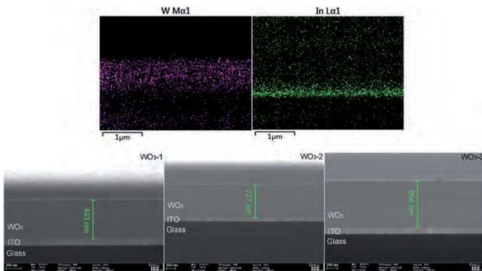
Fig. 7 Typical cross-view EDS-elemental mapping and SEM image of the FIB-cut sample for disassembled cathodic \text{WO}_3 EC films.
