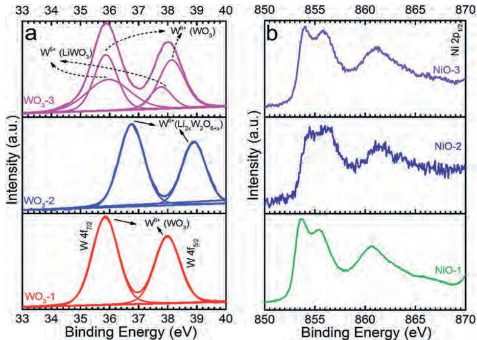
Fig. 12 XPS detail spectra for disassembled non-cycled and cycled (a) cathodic ( \text{WO}_3 -1 and \text{WO}_3 -2, \text{WO}_3 -3 respectively) and (b) anodic EC (NiO-1 and NiO-2, NiO-3 respectively) films.
