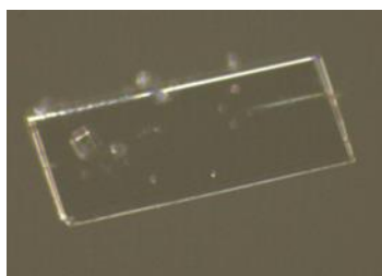
Figure 1. Picture of a single crystal of [\text{Y}(\text{Haobtc})(\text{H}_2\text{O})_2\cdot 2\text{H}_2\text{O}]_\infty
