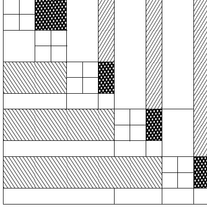
Figure 2: All updates at the third recursion level at step 9. The figure indicates the locations of U_{23} , L_{21} , and U_{13} .
