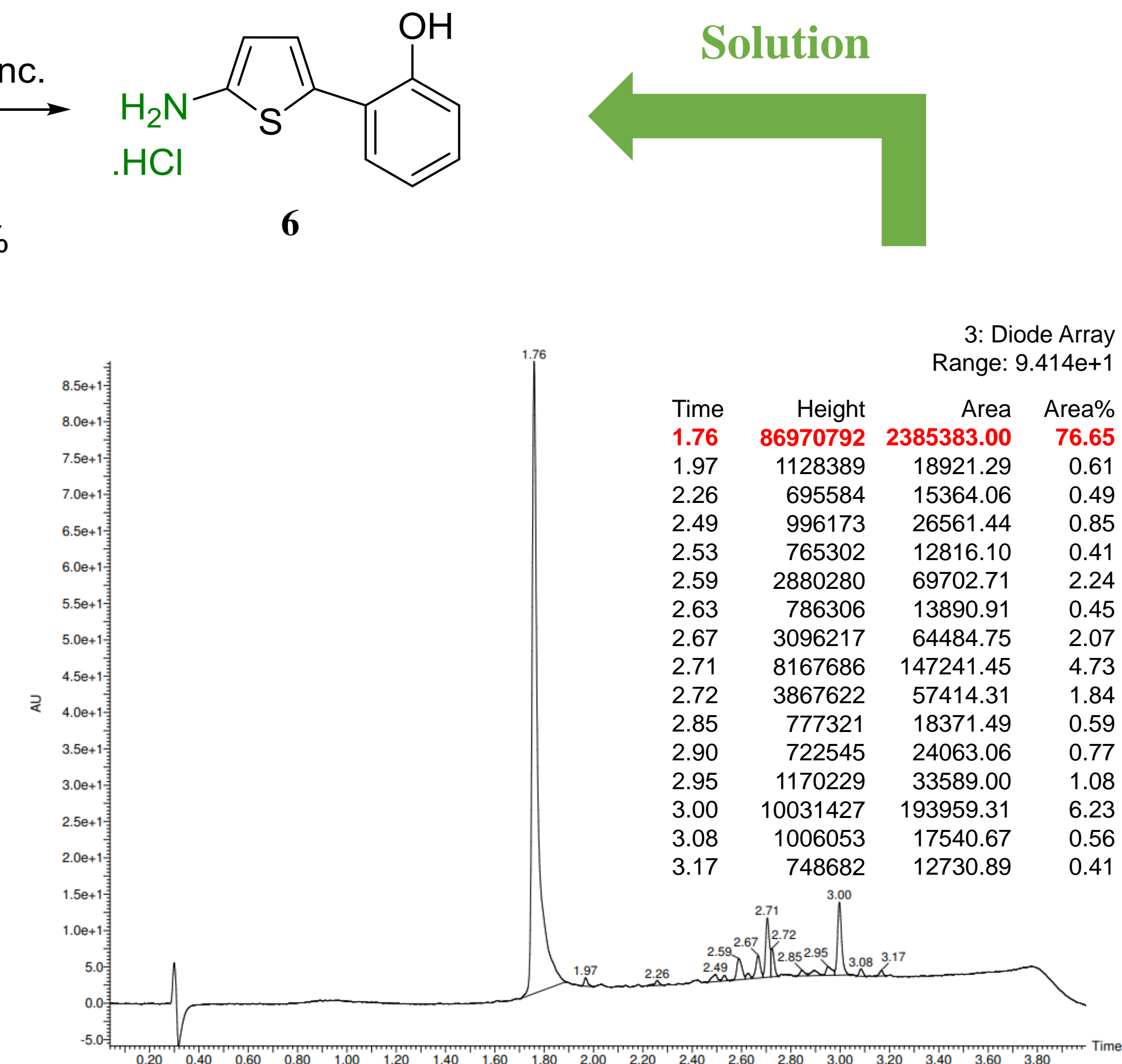
Scheme 2: Synthesis of amino thiophene derivatives
