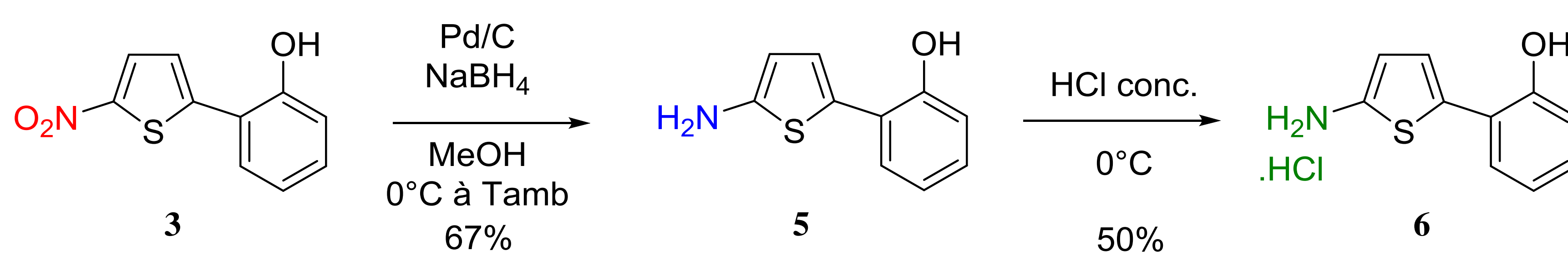
Scheme 2: Synthesis of amino thiophene derivatives
