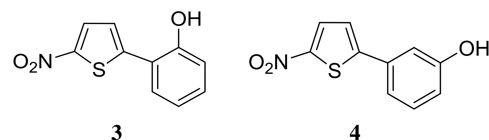
Figure 1: Structure of molecule 3 and 4
