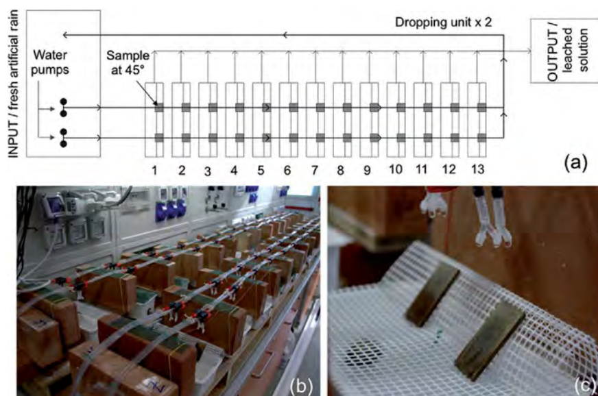
Fig. 1. (a) Schematic mode for a large-scale production of dropping test samples and (b) general view of the dropping system; (c) detail showing the quaternary bronze samples ( 45^\circ ) during ageing exposed at 45^\circ .
