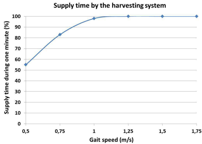
Figure 22. Supply time by the harvesting system
