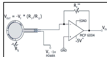
Figure 3. A401 sensor and its electronic conditioning
