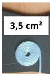
Figure 4. Winding of silicone tube and MS4525-1PSI sensor
