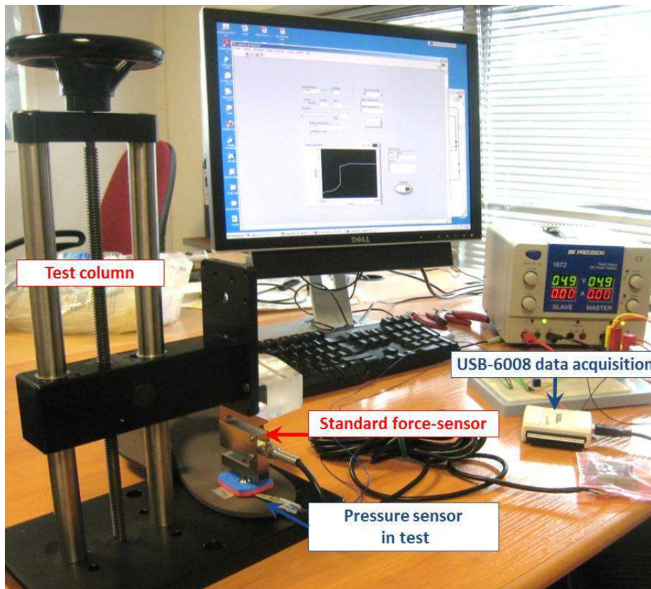
Figure 5. Overview of the test bench produced
