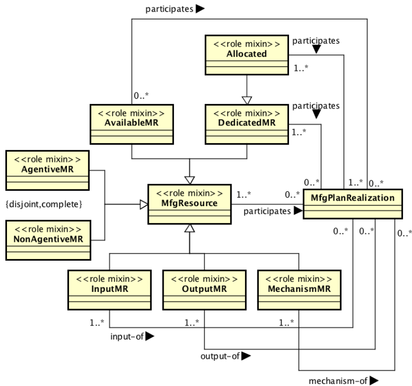
Fig. 2. High-level taxonomy of manufacturing resources
