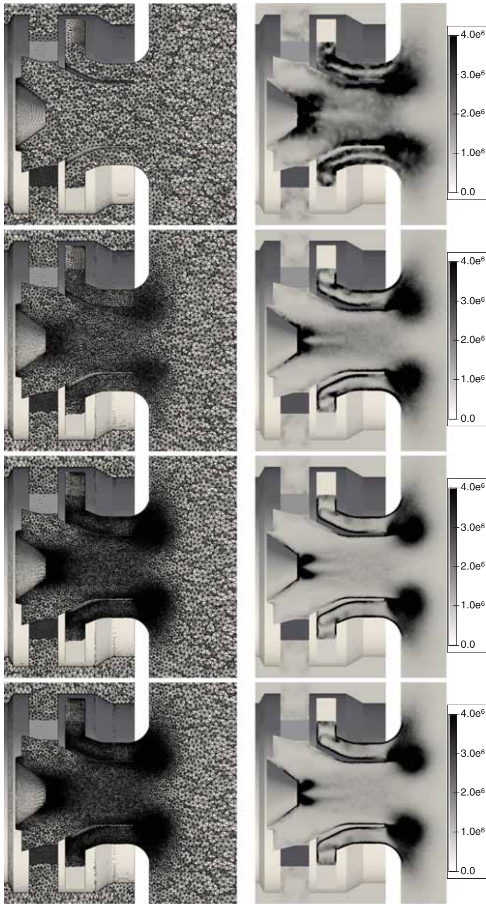
Fig. 12 \dot{m} = 4.29 \text{ g} \cdot \text{s}^{-1} case: meshes ( left ) and fields of \bar{\Phi} in \text{W} \cdot \text{m}^{-3} ( right ) for the coarse, AD 1, AD 2 and AD 3 meshes in the central plane of the swirler, from top to bottom , respectively
