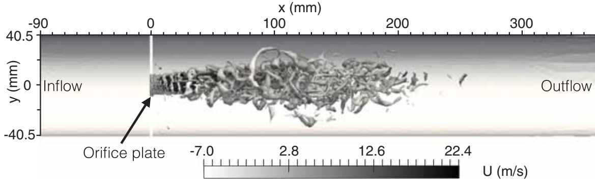
Fig. 4 LES of the orifice-plate at \dot{m} = 3.55 \text{ g} \cdot \text{s}^{-1} . The instantaneous flow is represent using Q-criterion Q = 1.62(U_j/D_j)^2 colored by axial velocity, on mesh AD 2
