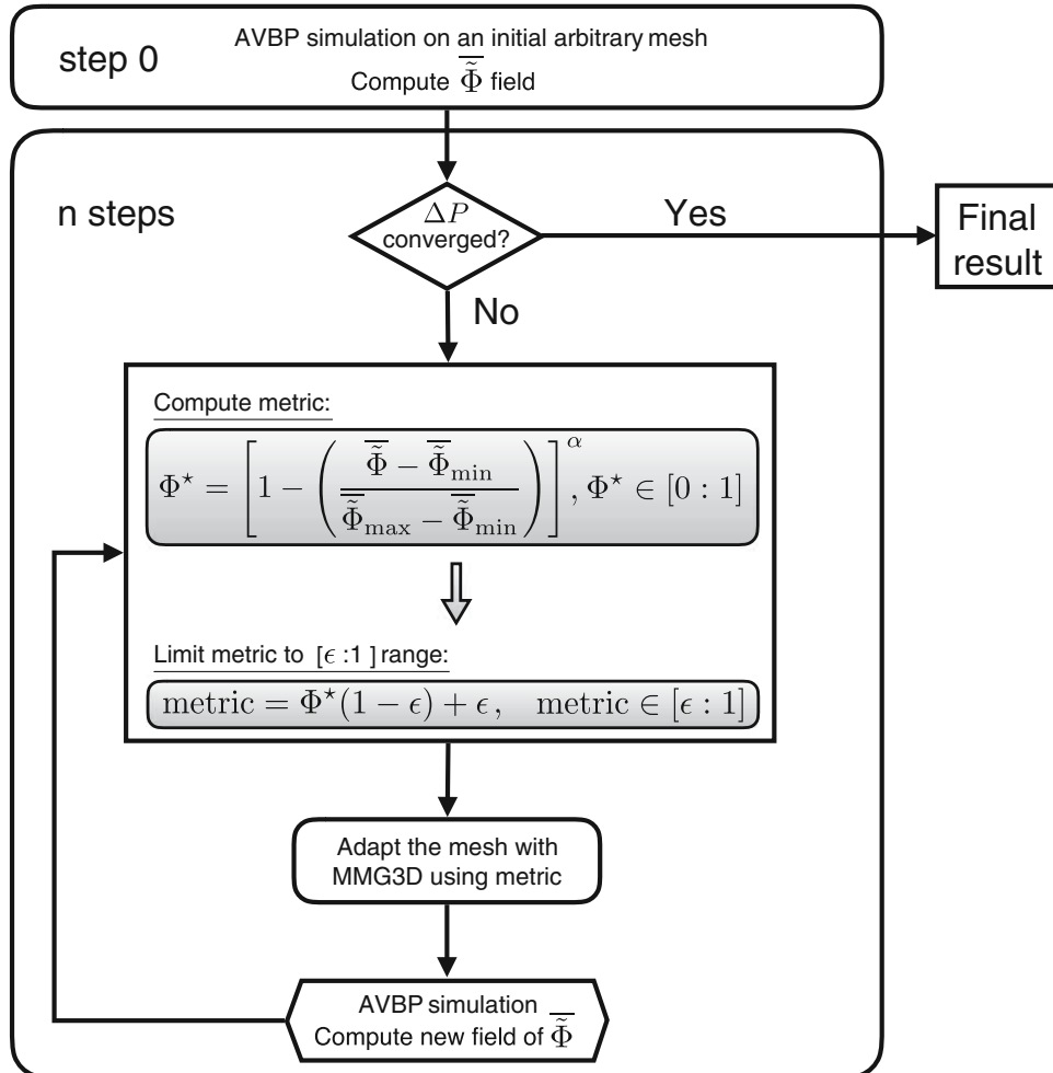
Fig. 1 Mesh adaptation procedure
