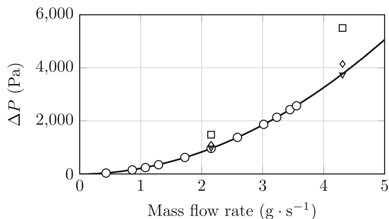
Fig. 9 Pressure loss evolution through the swirler: experimental data (○), fit function (—), LES results for the coarse (□), AD 1 (◇) and AD 2 (▽) meshes
