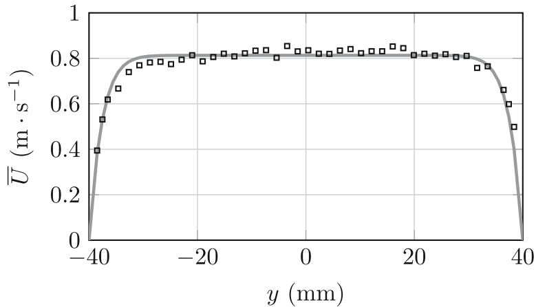
Fig. 10 \dot{m} = 4.29 \text{ g} \cdot \text{s}^{-1} case: mean axial velocity profile inside the plenum at x = -90 \text{ mm} from hot-wire measurement ( \square ), fit function ( \text{—} ) used as inlet condition in the LES
