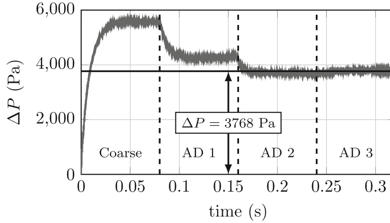
Fig. 11 \dot{m} = 4.29 \text{ g} \cdot \text{s}^{-1} case: Evolution of the pressure loss computed with LES as a function of time and comparison with the target experimental value ( straight solid line ). The pressure signal is recorded in the upstream plenum at the wall ( x = -50 \text{ mm} and r = 40.5 \text{ mm} ). The mesh is refined by the AVBP-MMG3D three times during the whole procedure
