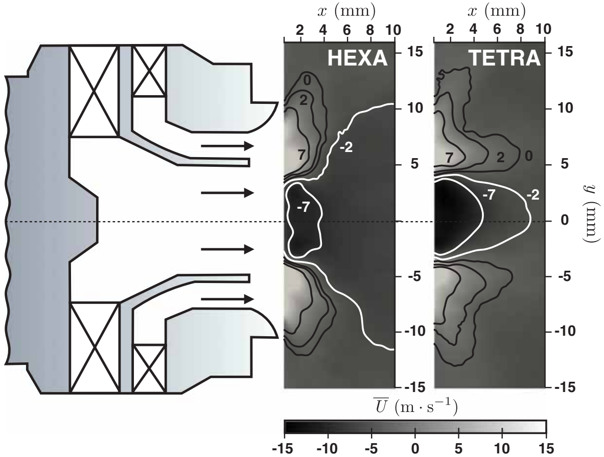
Fig. 18 Comparison of the mean axial velocity from LES on hexahedral H 2 mesh ( center ) and AD2 tetrahedral mesh ( right ) for the \dot{m} = 4.29 \text{ g} \cdot \text{s}^{-1} case. A schematic representation of the swirl injector is depicted on the left . White lines denotes negative mean velocity contours at -7 and -2 \text{ m} \cdot \text{s}^{-1} . Positive and zero mean velocity contours of 7 , 2 and 0 \text{ m} \cdot \text{s}^{-1} are shown with black line
