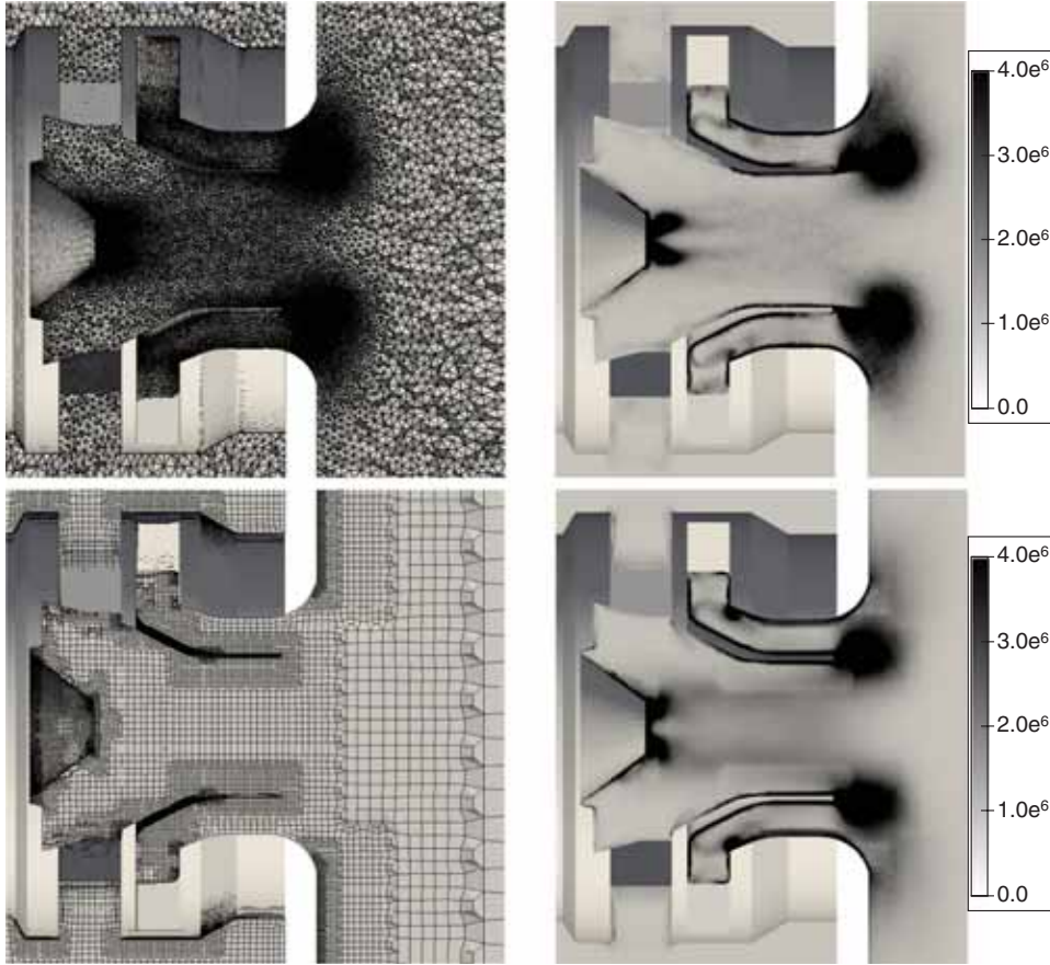
Fig. 17 \dot{m} = 4.29 \text{ g} \cdot \text{s}^{-1} case: meshes ( left ) and fields of \bar{\Phi} in \text{W} \cdot \text{m}^{-3} ( right ) for the tetrahedral AD 2 ( up ) and hexahedral H 2 ( bottom ) meshes
