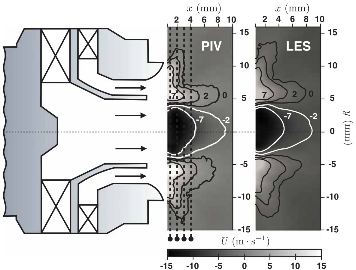
Fig. 13 Comparison of the mean axial velocity from PIV measurement ( center ) and LES on AD2 mesh ( right ) for the \dot{m} = 4.29 \text{ g} \cdot \text{s}^{-1} case. A schematic representation of the swirl injector is depicted on the left . White lines denotes negative mean velocity contours at -7 and -2 \text{ m} \cdot \text{s}^{-1} . Positive and zero mean velocity contours of 7 , 2 and 0 \text{ m} \cdot \text{s}^{-1} are shown with black line . Dashed-lines identify the position of the measurement cross-sections downstream of the exit plane at x = 1, 2, 3, 4 \text{ mm}
