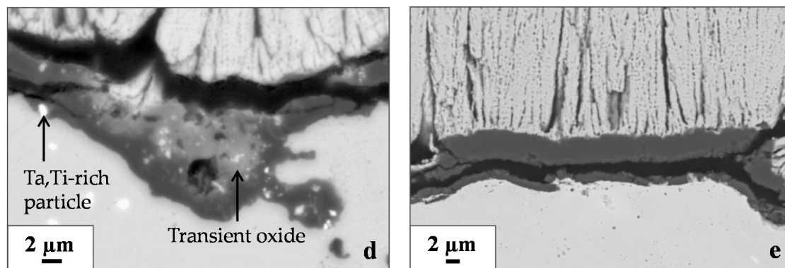
Figure 3. Cross-sections of (a,c,e) AM3-Trib-Pt/1 TBC system after 290 cycles; and (b,d) AM3-Trib TBC system after 36 cycles. Thermal cycles of 1 h at 1100 °C, with a high flow air cooling. (a) Presence of many corn kernel defects due to a rough bond-coating surface before thermal barrier deposition; (b) Cracking at thermally grown oxide (TGO)/thermal barrier interface; (c) Thermal barrier still adherent to the TGO, except at corn kernel areas; (d) TGO not only composed of alumina; (e) Only alumina detected in the TGO. SEM images in BSE mode.
