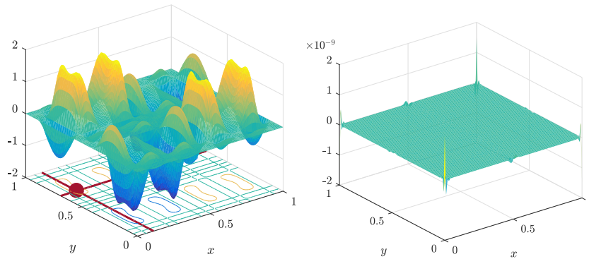
(c) Residual after 2 modes r_2 and interpolation index \rho_2 = (0.11, 0.69) (d) Last residual, after 14 terms: r_{14}
