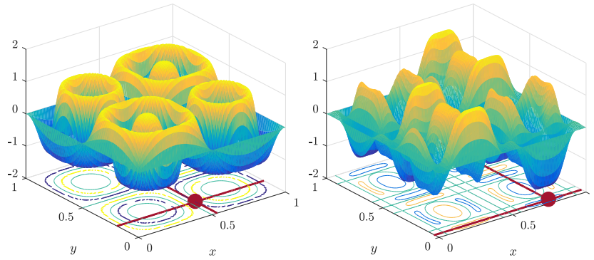
(a) Initial residual r_0 and interpolation index \rho_0 = (0.54, 0.19) (b) Residual after 1 mode r_1 and interpolation index \rho_1 = (0.78, 0.04)
