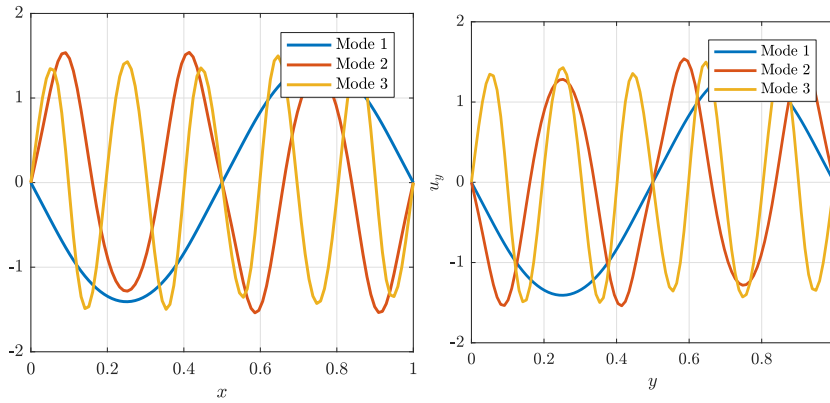
(b) First 3 x-dir. modes: \{\mathbf{w}_0^m\}_{m=1}^3 (c) First 3 y-dir. modes: \{\mathbf{w}_1^m\}_{m=1}^3
