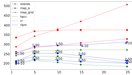
Figure 4. Normalised MI of the evaluated strategies in ordinate for the three maps and the population sizes of agents in abscissa.
