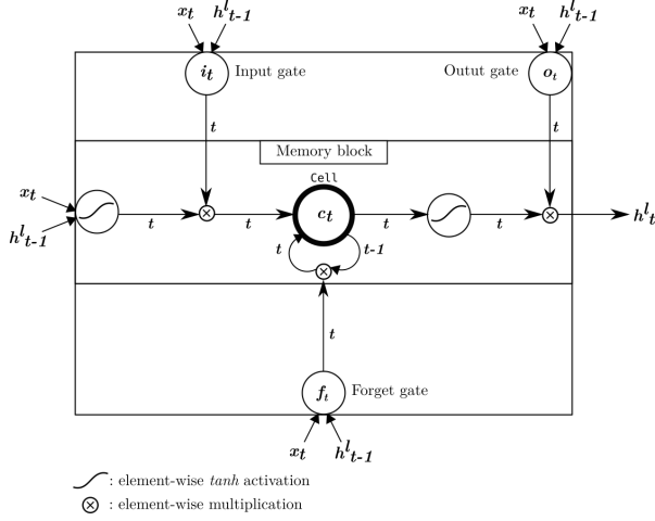
Figure 1. Layered LSTM unit: the core component of the LSTM architecture.
