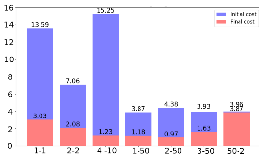
Figure 3. Costs averaged over the maps and numbers of agents for each architecture.
