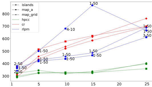
Figure 5. Normalised QMI of the evaluated strategies in ordinate for the three maps and the population sizes of agents in abscissa.
