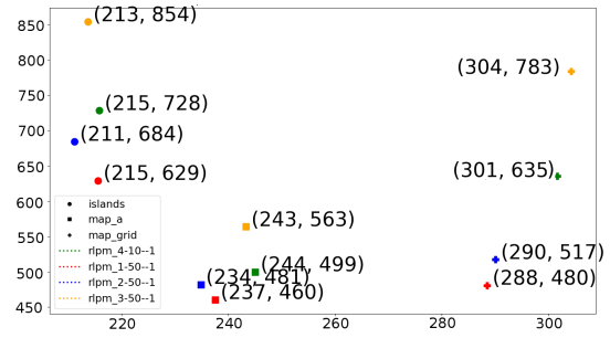
Figure 6. Criterion space of MI and QMI.
