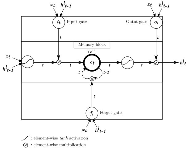
Figure 1. Layered LSTM unit: the core component of the LSTM architecture.
