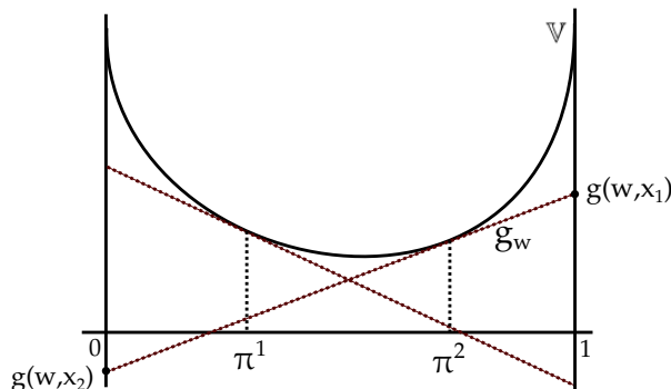
Figure 1: Actions w constructed from subgradients on different priors.
