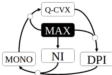
Figure 3: Equivalence of axioms under MAX. The merging arrows indicate joint implication: for example, \text{MAX} \wedge \text{Q-CVX} implies DPI. Compare with Figure 2.
