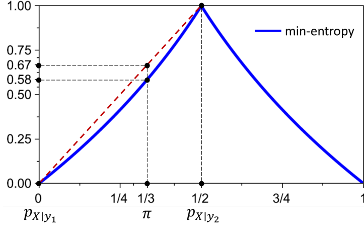
Figure 4: A picture showing how posterior min-entropy can be greater than prior min-entropy. Pushing prior \pi = (1/3, 2/3) through channel C gives hyper [\pi \triangleright C] with outer (1/3, 2/3) and inners p_{X|y_1} = (0, 1) and p_{X|y_2} = (1/2, 1/2) . So H_\infty(\pi) = -\log_2 2/3 \approx 0.58 and \hat{H}_\infty[\pi \triangleright C] = 1/3 \cdot 0 + 2/3 \cdot 1 \approx 0.67 .
