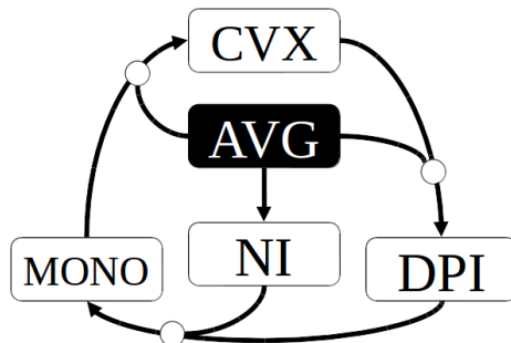
Figure 2: Equivalence of axioms under AVG . The merging arrows indicate joint implication: for example, \text{AVG} \wedge \text{CVX} implies DPI .
