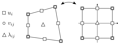
Figure 1. The 2D second gradient finite element 36
