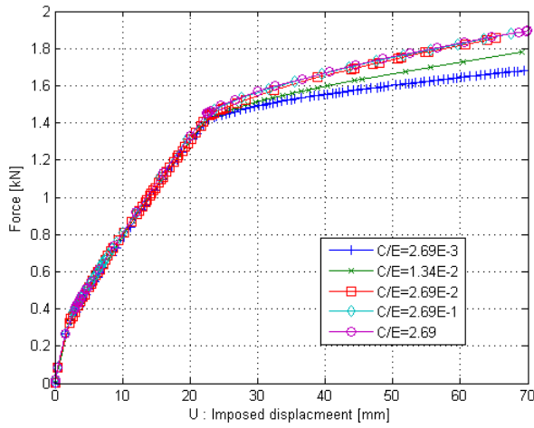
Figure 8. Three points bending test: reaction force vs. imposed displacement for different normalized penalty factors
