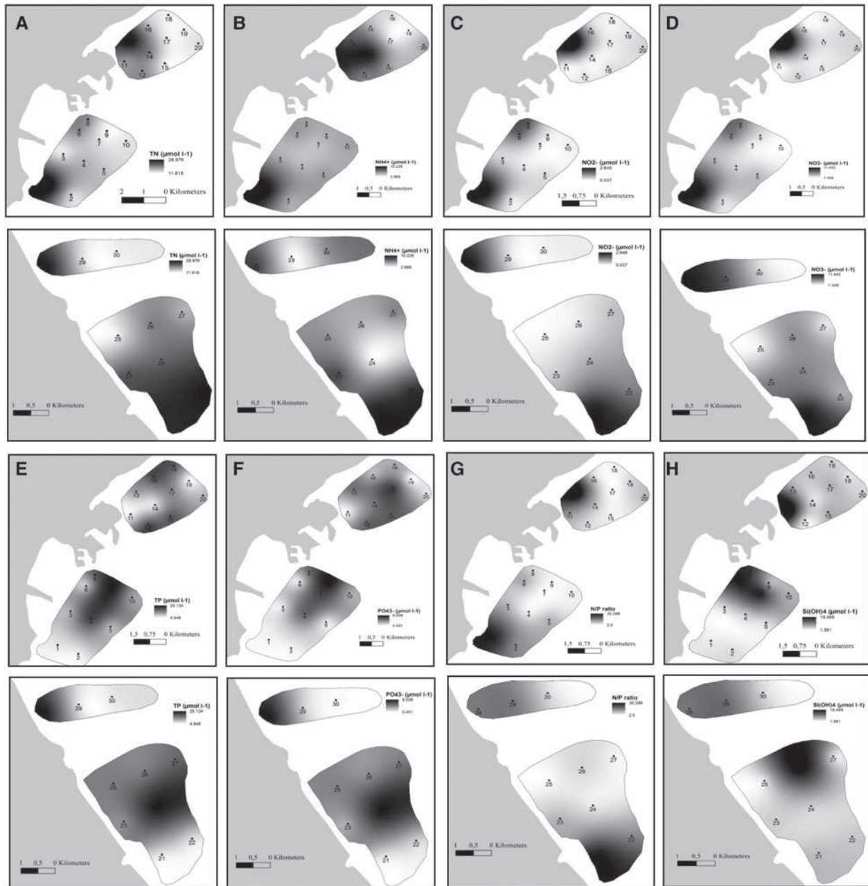
Fig. 3. Spatial variation of nutrient compounds, i.e. total nitrogen (T-N) (A), ammonium ( \text{NH}_4^+ ) (B), nitrite ( \text{NO}_2^- ) (C), nitrate ( \text{NO}_3^- ) (D), total phosphate (T-P) (E), orthophosphate ( \text{PO}_4^{3-} ) (F), N/P ratio (G) and silicate ( \text{Si(OH)}_4 ) (H) in stations sampled in the northern and southern coastal areas of Sfax and the Ghannouch area during autumn (October–November 2014).
