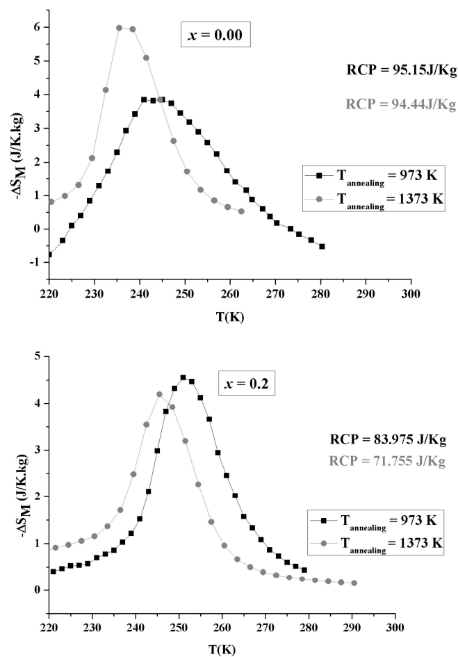
Figure 5. Temperature dependence of the magnetic entropy change ( -\Delta S_M ) measured for an applied magnetic field of 2 T for x = 0.00 and 0.2 samples annealed at 1373 and 973 K. RCP: relative cooling power.
