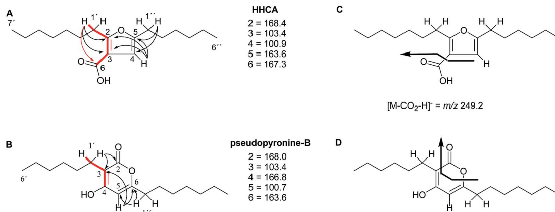
Fig. 2 The putative (A) and revised (B) structure of 2-heptyl-5-hexylfuran-3-carboxylic acid (HHCA; 3 ), which was reported as pseudopyronine-B. Arrows in A and B indicate ^1\text{H} - ^{13}\text{C} HMBC correlations; red color indicates ^4J_{\text{H,H}} coupling of interest. Panel C shows the putative explanation of the MS/MS fragmentation of HHCA in negative mode; fragmentation of the pseudomolecular ion [\text{M} - \text{H}]^- = m/z 293.2 . Panel D provides the correct true explanation for the observed MS/MS fragment. The arrow with the solid line in (C) and (D) directly shows the decarboxylation process.
