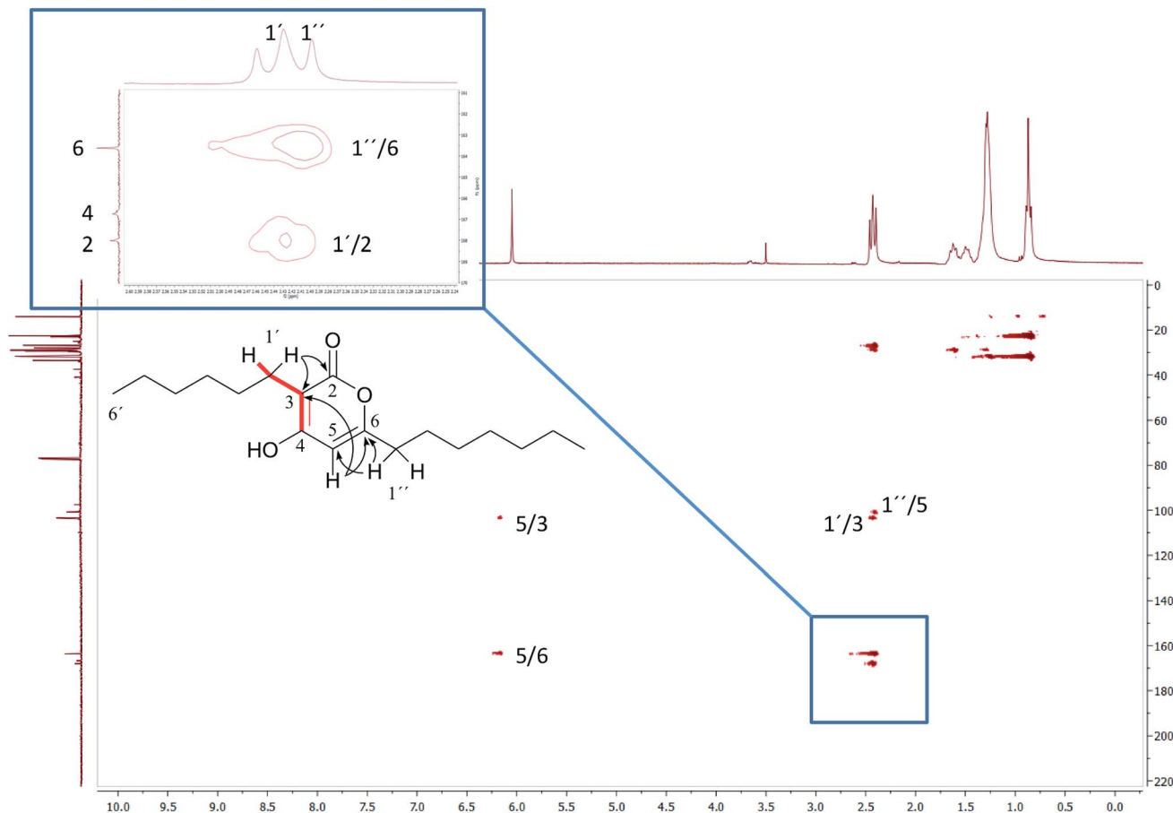
Fig. 3 ^1\text{H} - ^{13}\text{C} HMBC NMR spectrum of pseudopyronine B ( 4 ); insert show details of the 160 ppm region.
