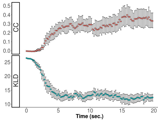
Figure 5: Saliency maps similarities between starting rotation condition groups as a function of time. Similarity measures reported: CC (red) and KLD (blue). Error bars report confidence intervals (95%).
