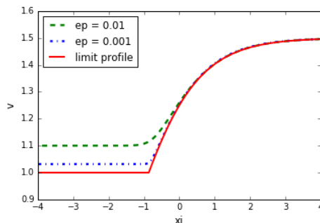
FIGURE 3. Asymptotic behavior of the profiles \mathbf{v}_\varepsilon joining the end-states v_-^\varepsilon = 1 + \varepsilon^{1/\gamma} and v_+ = 1.5 .
