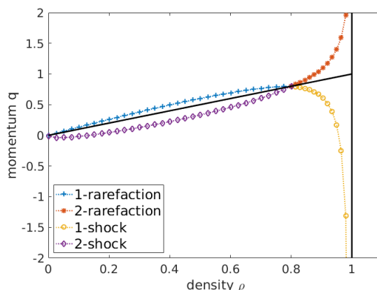
FIGURE 2. Rarefaction and shock curves for the reference left state (\rho_l, q_l) = (0.8, 0.8) and parameters \varepsilon = 0.01 , \gamma = 2 in the pressure law.
