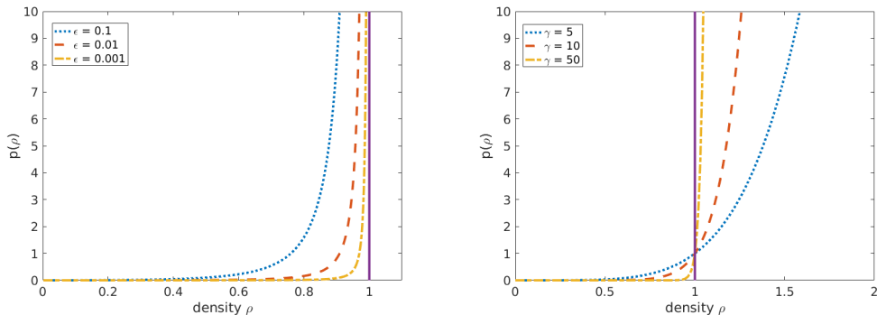
FIGURE 1. Different approximate pressures. On the left: singular pressures p_\varepsilon = \varepsilon \left( \frac{\rho}{1-\rho} \right)^\gamma ( \gamma = 2 ) corresponding to the soft congestion approach. On the right: power laws p_n(\rho) = a\rho^{\gamma_n} ( a = 1 ) corresponding to the penalty method.
