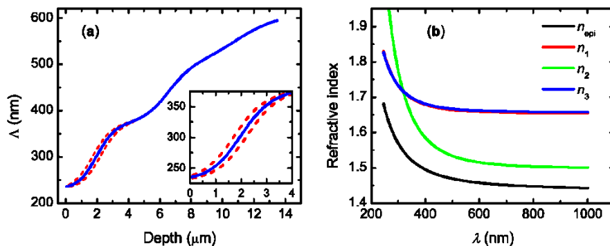
Figure 2. (a) Pitch profile across the exocuticle of C. chrysargyrea determined from the regression analysis of Mueller-matrix data. (b) Refractive indices of epicuticle ( n_{epi} ) and principal components ( n_1 , n_2 , n_3 ) of the anisotropic slices modelling the exocuticle. The insert in (a) shows the pitch variation near the cuticle surface accounting for depolarization at wavelength shorter than 550 nm. [10]. © The Authors 2018.
