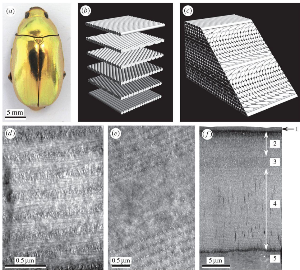
Figure 3. (a) C. resplendens photographed under unpolarized illumination. (b) An exploded view of a helicoidal set of fibrils ‘planes’. (c) A view of a section of helicoidal stack. The oblique cut reveals Bouligand arc patterns in the arrangement of fibrils. A full helicoidal pitch is shown. (d) TEM image showing details of an oblique section of the elytron. (e) TEM image showing details of a section perpendicular to the cuticle surface. The unidirectional layer or birefringent retarder is shown as the uniform band extending across the center of the image. Cholesteric regions are disposed above and below. (f) TEM of a perpendicular section through the outer part of the cuticle, indicating its component regions: 1: epicuticle; 2: upper cholesteric region; 3: unidirectional (nematic) layer; 4: lower cholesteric region; 5: endocuticle (portion). Regions 2 to 4 form the exocuticle [15]. © The Authors 2017.
