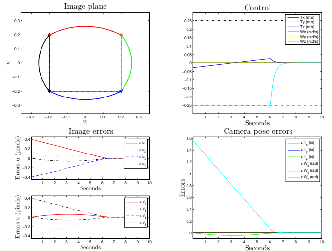
Fig. 6. N_p = 10 and Q = I
