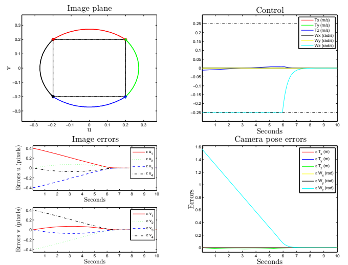
Fig. 7. N_p = 10 and Q = Q(t)
