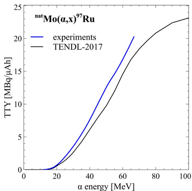
Figure 7. TTY for {}^{97}\text{Ru} production via {}^{\text{nat}}\text{Mo}(\alpha,x) on metallic {}^{\text{nat}}\text{Mo} target. The experimental curve (blue) is calculated using the cross-section from this work (above 40 MeV) and the data provided by [3,20] below 40 MeV.
