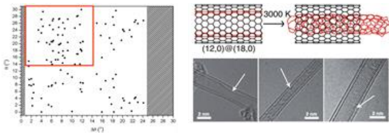
Figure 3 : Left: Statistical analysis plotting outer helicity versus helicity difference between outer and inner tubes: favored (red square) and non observed (dashed areas) configurations are marked . Right top : Relaxed configuration of forbidden DWNT after MC simulation. (c) Defected DWNTs observed experimentally where the inner tube diameters locally decrease (white arrows) as found in MC simulations.
