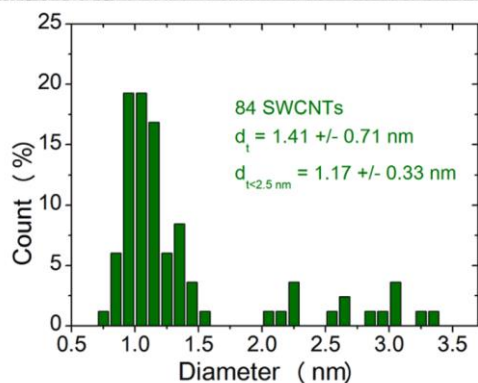
Figure 2: typical TEM image of the transferred diameter-sorted SWCNTs, with the measured diameters instructed in white; diameter distribution histogram extracted from the measurement of the diameters of 84 SWCNTs on random locations on the grid.
