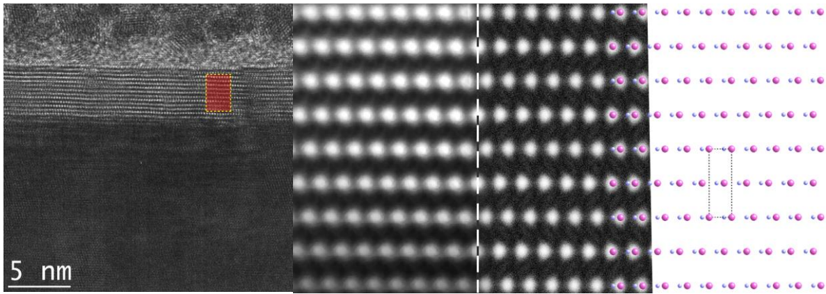
Figure 2 : (left) HRTEM image of the cross section of a BN film grown on a Ni(111) surface ; zoom on stacking sequence :(right) filtered image, simulated TEM image with JEMS and AB stacking representation
