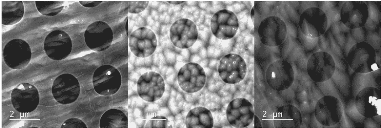
Figure 1 : HAADF image of BN deposit transferred on TEM grids. The 3 different images correspond to different morphologies of the film related to the orientation of the Ni grains.
