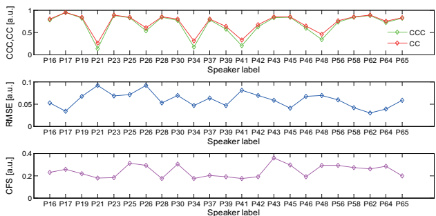
Fig. 4. Performance obtained during the training of each SSRM for the valence dimension (from top to bottom): concordance correlation coefficient (CCC), Pearson’s correlation coefficient (CC), root mean square error (RMSE), and correlation-based feature selection (CFS).
