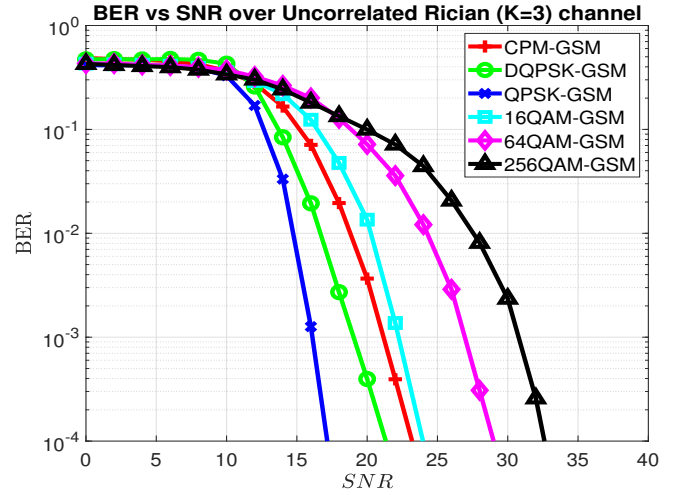
Fig. 5. BER vs SNR for various systems over uncorrelated Rician channel
