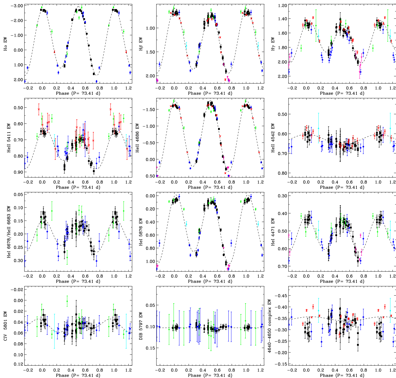
Figure 4. Rotationally phased EW measurements for selected lines in the spectrum of CPD -28^\circ 2561. Least-squares sinusoidal fits are shown for those lines with statistically significant EW variability. In the bottom row, we also show measurements of the \lambda 5797 DIB as an example of an intrinsically non-variable feature. In these figures, the ESPaDOnS measurements are black squares, the HARPS measurement is the cyan upwards facing triangle, the FEROS measurements are the blue circles, the LCO/echelle measurements are the green diamonds, the CAS measurements are the pink downward facing triangles, and the B&C measures are red crosses.
