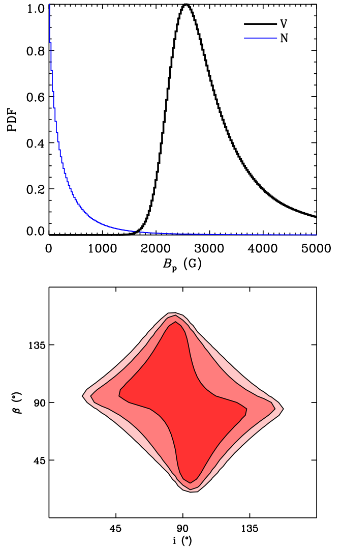
Figure 12. Magnetic field polar strength (upper frame) and geometry ( i , \beta ) (lower frame) constraints derived from modelling of Stokes V profiles.
