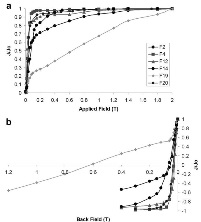
Fig. 3. a) IRM acquisition and b) IRM back-field curves of selected samples.
