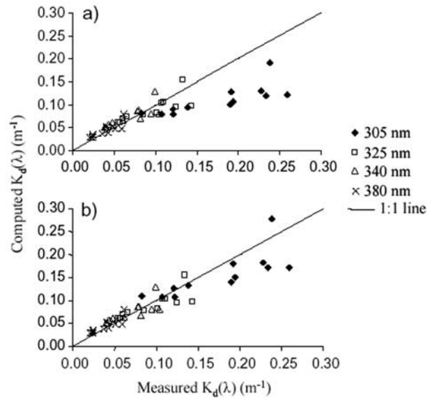
Figure 3. Comparison between measured and computed K_d(\lambda) at 305 nm (UV-B), and 325, 340 and 380 nm (UV-A) between 0 m and 15 or 30 m for the stations of the south east Pacific, except UPW ( n = 12 ). Measured K_d(\lambda) were derived from in situ optical measurements whereas computed K_d(\lambda) were calculated from UV-extended IOP and RT models. The UV-extended IOP model was used with in situ surface Chl a concentration (see Table 1) as input parameter assuming the Case 1 water model. Different values of CDOM absorption spectral slope coefficient ( S ) were used: (a) S = 0.017 \text{ nm}^{-1} over the UV spectral domain (at 305, 325, 340 and 380 nm) as proposed by Kopelevich et al. [1989] and used by Vasilkov et al. [2005] in the North Pacific waters and (b) S = 0.017 \text{ nm}^{-1} at 325, 340, 380 nm and S = 0.023 \text{ nm}^{-1} at 305 nm, combined from two separate one- S -value extrapolations. For Figures 3a and 3b, the determination coefficient ( r^2 ) of the linear correlation was 0.60, p < 0.01 at 305 nm, 0.67, p < 0.01 at 325 nm, 0.65, p < 0.01 at 340 nm and 0.76, p < 0.001 at 380 nm.
