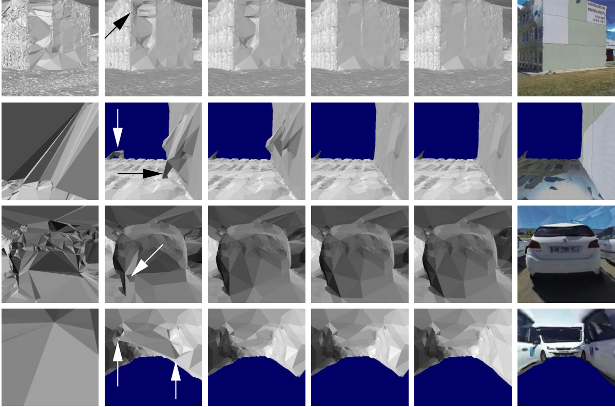
Figure 16: Handles of M_0 and their removals by M_1 , M_2 and M_3 . From left to right: \partial F , M_0 , M_1 , M_2 , M_3 , and texture of M_3 . There are views from outside and from inside of a building corner (rows 1&2) and a car (rows 3&4). The arrows are pointing to handles removed by M_1/M_2/M_3 .
