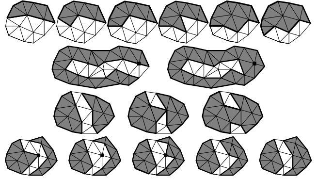
Figure 2: Local operations in the 2D case. (Tetrahedra are replaced by triangles.) From top to bottom: Shelling (Sh.), Topology Extension (T.E.), Force-Repair (F.R.) and Shrink-Grow (S.G.). Every line shows successive values of O in gray. Sh. adds one tetrahedron at once to O and g does not change. T.E. adds all tetrahedra around a vertex to O so that g can increase. F.R. adds tetrahedra, a singularity is first created and then removed. S.G. first removes then adds tetrahedra to O .
