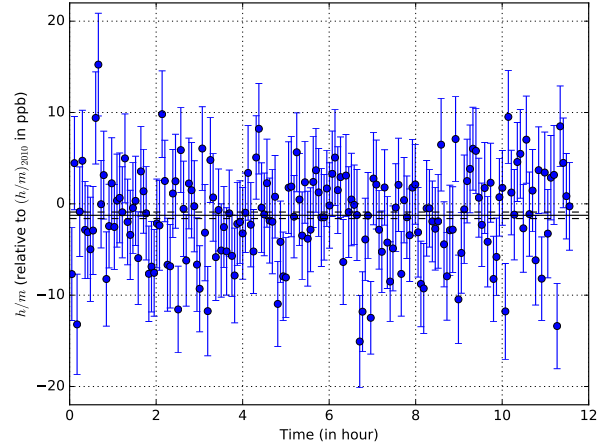
Figure 11: A set of 180 measurements of the ratio h/m_{\text{Rb}} obtained during 12 hours of integration time. Raw data are plotted relative to the value of (h/m)_{2010} = 4.591\,359\,2729\,(57) \times 10^{-9} \text{ m}^2\text{s}^{-1} . No correction of systematic effects was applied to this set of data.
