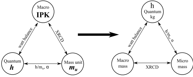
Figure 3: In the current SI, the ratio h/m_u provides a direct comparison between the watt balance experiment and the XRCD experiment. In the future SI this ratio would achieve the Mise en pratique of the kilogram at the atomic scale and at the macroscopic scale using the XRCD method.
