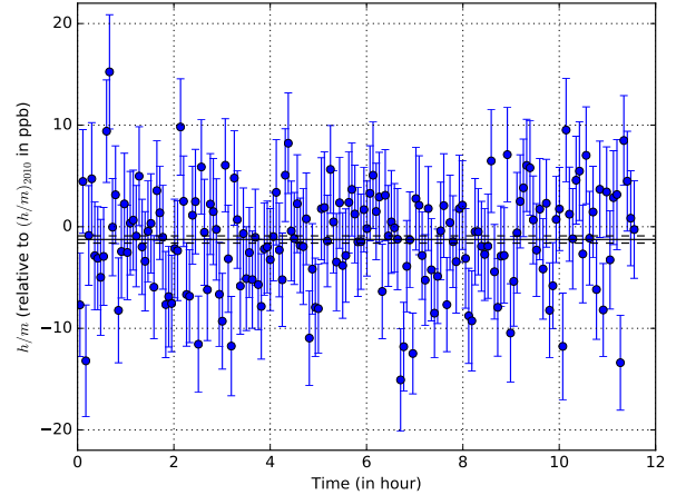
Figure 11: A set of 180 measurements of the ratio h/m_{\text{Rb}} obtained during 12 hours of integration time. Raw data are plotted relative to the value of (h/m)_{2010} = 4.591\,359\,2729(57) \times 10^{-9} \text{ m}^2\text{s}^{-1} . No correction of systematic effects was applied to this set of data.
