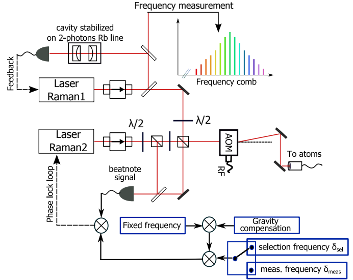
Figure 8: The optical setup of the Raman beam used to perform the atomic interferometer. The two laser diodes are stabilized using an interference-filter-stabilized extended cavity. They are phase-locked. The frequency of one Raman laser is stabilized on an ultra-stable cavity and measured with a femtosecond comb.
