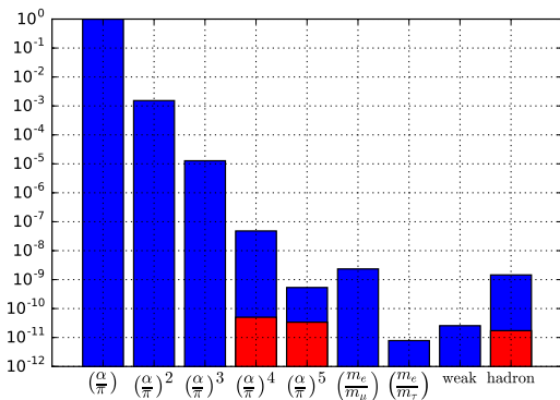
Figure 1: Relative contributions to the electron anomaly of the different terms of equation 2, in red their uncertainties.
