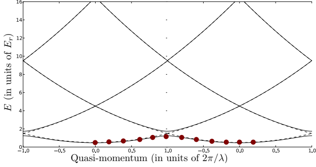
Figure 5: Visualisation of a Bloch oscillation. The atoms are placed in a periodic potential and therefore present a band structure. Eigenstates can be described by the band index and the quasimomentum (x-axis). When an atom prepared in the first band is accelerated, its quasimomentum increases linearly. At the edge of the Brillouin zone (centre of the graph) the atom will follow adiabatically the fundamental band if the acceleration is not too strong. After one oscillation, the atom is back to the initial state.
