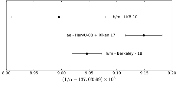
Figure 13: Zoom on the three best determinations of \alpha : the h/m_{\text{Rb}} measurement of LKB [1]; the measurement of a_e from Harvard [2] combined with the last calculation from Riken [10]; and the measurement of h/m_{\text{Cs}} from Berkeley [4].
