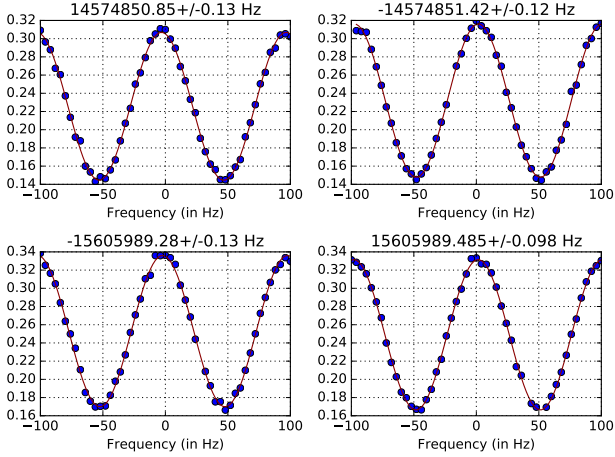
Figure 10: Typical set of four spectra used for the determination of h/m_{\text{Rb}} . The quantity N_2/(N_1 + N_2) , where N_1 and N_2 represent respectively the populations in hyperfine F = 1 and F = 2 state, is plotted versus the frequency difference \delta_{\text{sel}} - \delta_{\text{meas}} . The four spectra are recorded with 50 points each during 4 minutes in total. The measured position of the central fringe is indicated over each spectrum.
