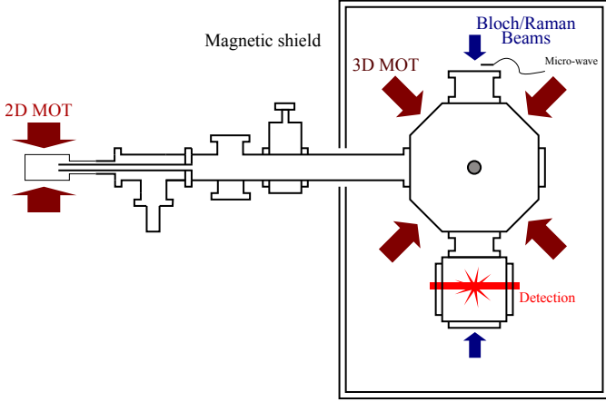
Figure 7: Schematic of the experimental setup used to measure h/m_{\text{Rb}} .
