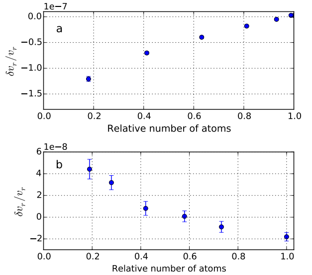
Figure 12: Systematic effect in the measurement of the atomic recoil due to noise in the optical field. We have plotted the measurement of the atomic recoil when we filter the atoms in a zone of relatively high intensity (plot a) or relatively low intensity (plot b). The x-axis represents the number of remaining atom from right (100%, no selection) to the left (strong selection).
