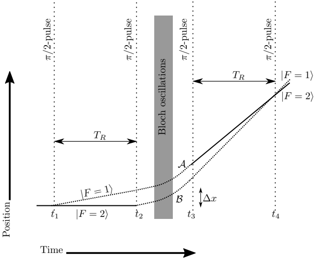
Figure 6: Schematic of the Ramsey-Bordé interferometer used to measure the recoil velocity. A sequence of four Raman \pi/2 pulses splits and recombines the atomic wavepacket in two paths (label \mathcal{A} and \mathcal{B} ). Between the second and third pulse, Bloch oscillations are used to accelerate the atoms.
