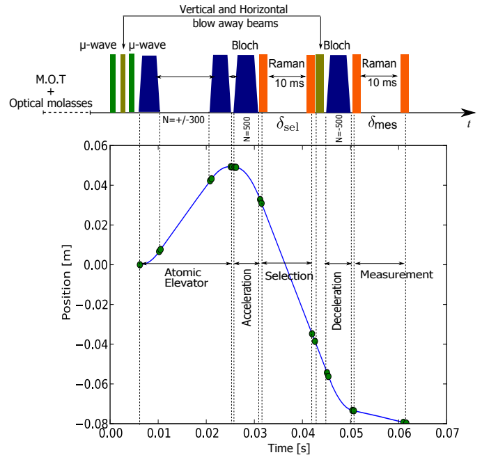
Figure 9: The pulses timing sequence and atomic trajectory during the measurement procedure.
