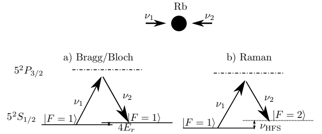
Figure 4: Atoms are shed with two counter propagating laser beam of frequency \nu_1 and \nu_2 . When they absorb and emit a photon, they acquire twice the recoil velocity. a) In the Bloch oscillation configuration (which is also the same for Bragg diffraction), \nu_1 \approx \nu_2 , the transition occurs between the same internal state. The difference between \nu_1 and \nu_2 accounts only for the Doppler shift induced by the recoil. b) In the Raman configuration, \nu_1 - \nu_2 is almost equal to the hyperfine splitting \nu_{\text{HFS}} , and the transition change the internal state.
