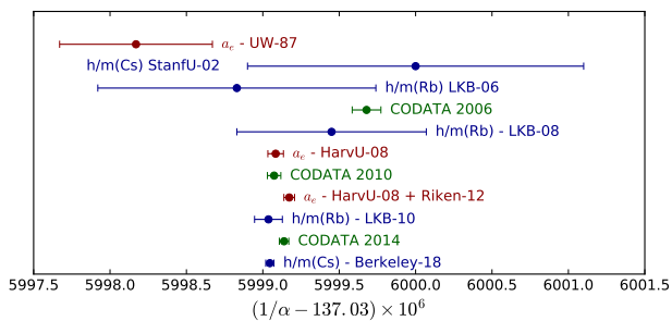
Figure 2: Comparison of different determinations of \alpha with uncertainties below 10^{-8} . In red, determinations from the magnetic moment of the electron, in blue from h/m_{\text{At}} and in green from the CODATA. UW: University of Washington [11]; LKB: Laboratoire Kastler Brossel (Paris) [12, 13, 1]; Berkeley [4]; HarvU: Harvard University [2]; Riken [3]; CODATA [14, 15, 16]
